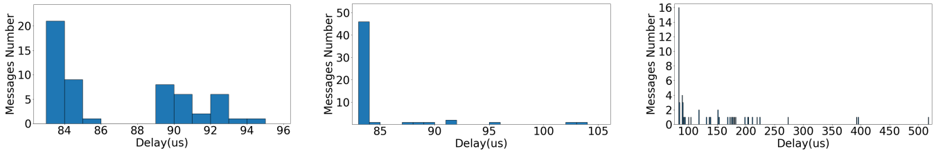
Fig. 2: End-to-end delay of AFDX traffic with a Poisson mean rate of 0.125ms for AFDX table scheduling (left), SPQ (center) and FIFO (right)
